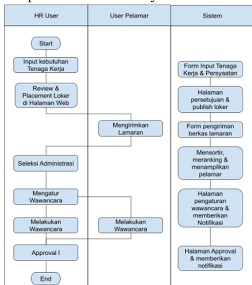
Gambar 2. Diagram Activity Admin
